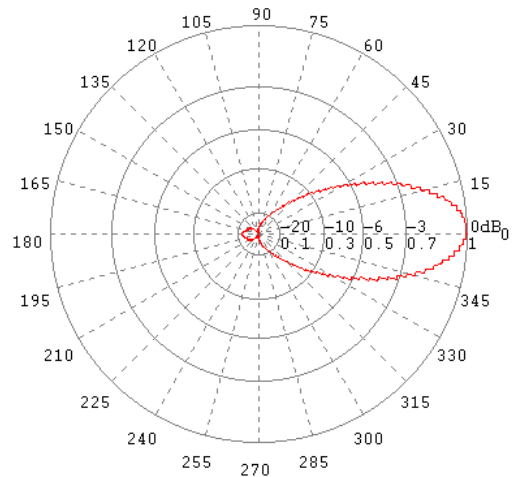
H-Ebene / H-Plane 2 GHz
