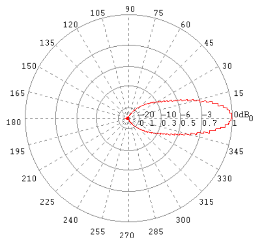
H-Ebene / H-Plane 3 GHz
