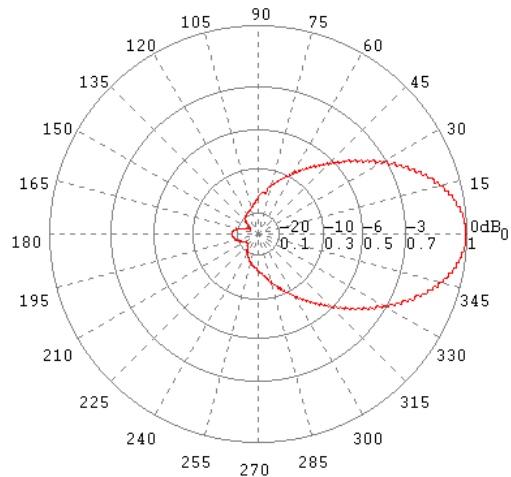
E-Ebene / E-Plane 1 GHz
