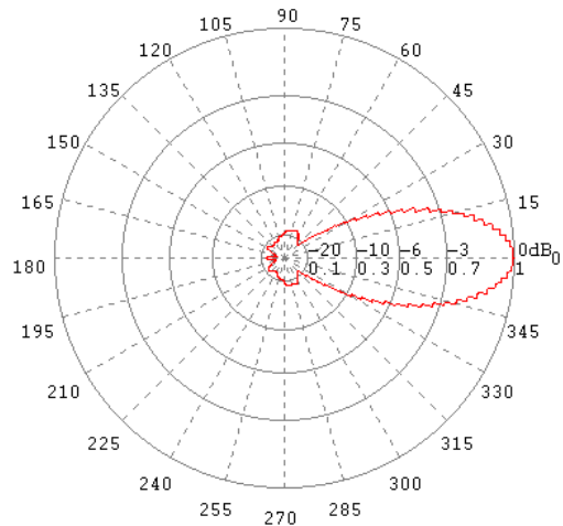
E-Ebene / E-Plane 2 GHz
