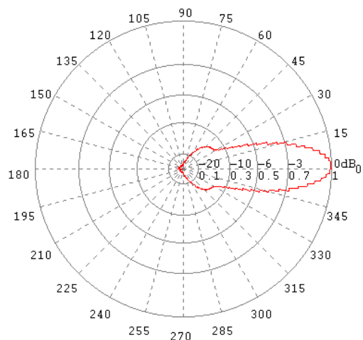
E-Ebene / E-Plane 3 GHz
