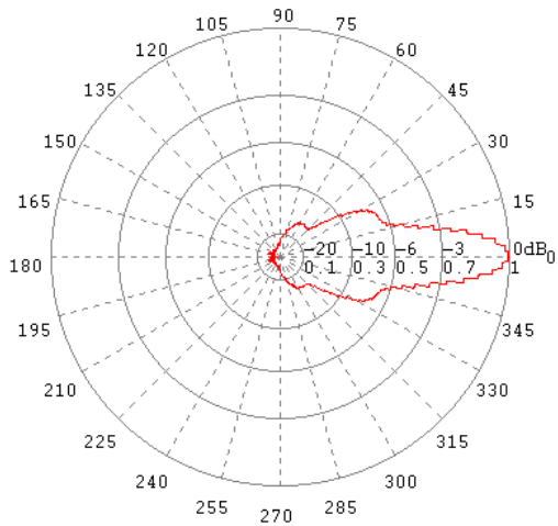
E-Ebene / E-Plane 4 GHz
