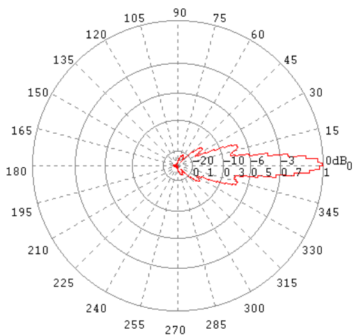
E-Ebene / E-Plane 6 GHz
